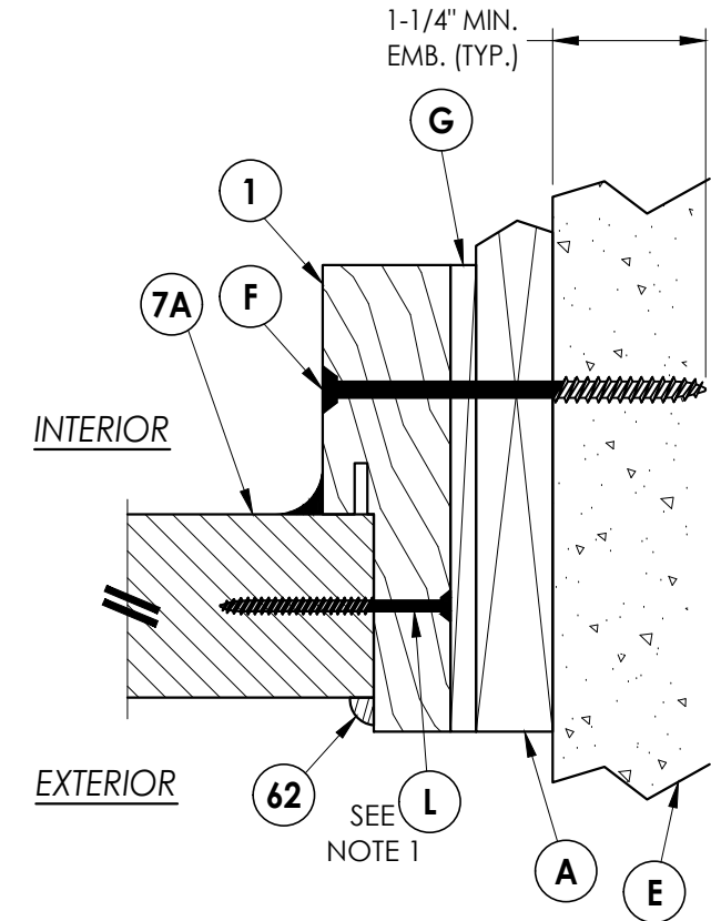
3/4 HORIZONTAL CROSS SECTION Shown w/1X sub-buck
