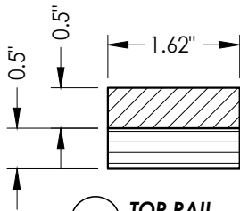
33 TOP RAIL
