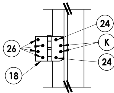
HINGE DETAIL 1
